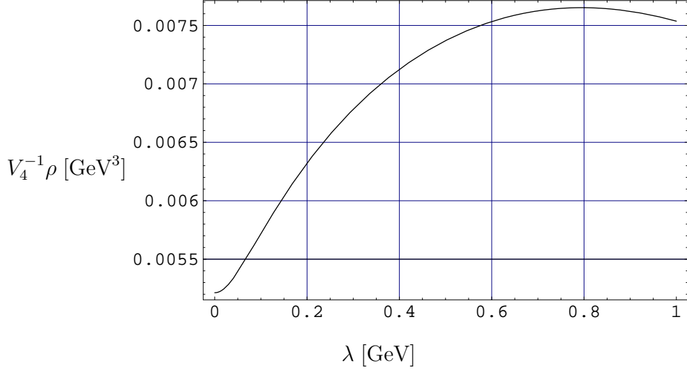
Figure 3: The spectral density \rho(\lambda) of the Dirac operator \tilde{D} computed in the linear \sigma -model with quarks. Note the suppressed zero on the scale for V_4^{-1}\rho .
